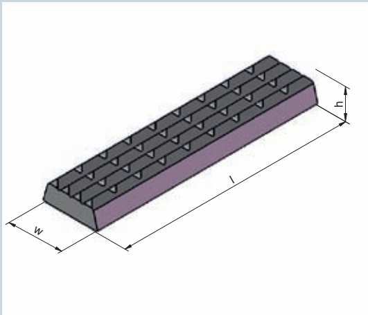
Diamond Tooth Tong Die:
